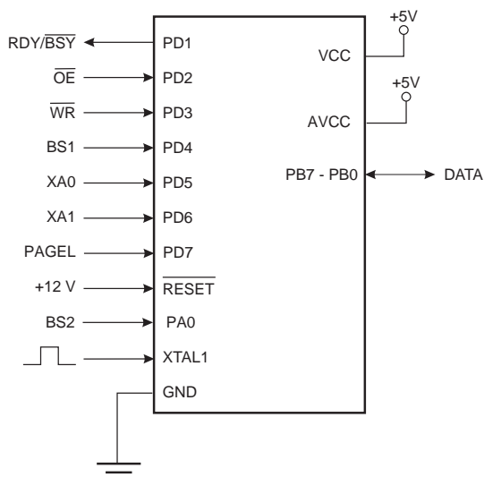
Figure 25-1. Parallel Programming (1)
