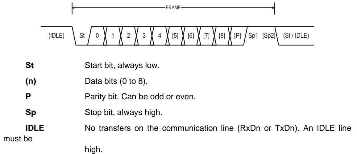
Figure 17-4. Frame Formats
