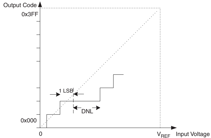
Figure 21-13. Differential Non-linearity (DNL)
