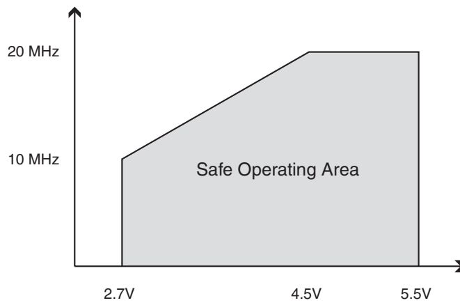
Figure 26-3. Maximum Frequency vs. V_{CC} , ATmega644
